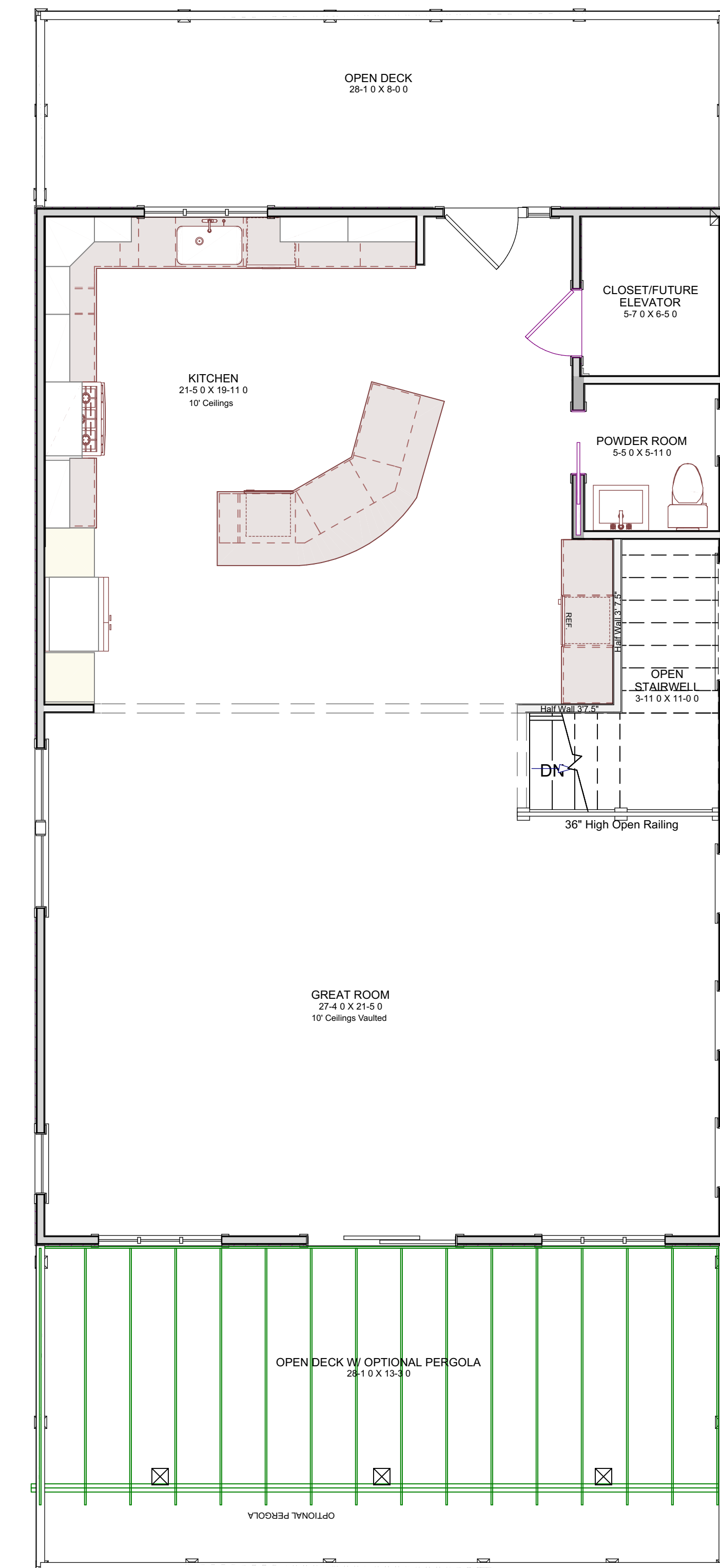
THIRD FLOOR
