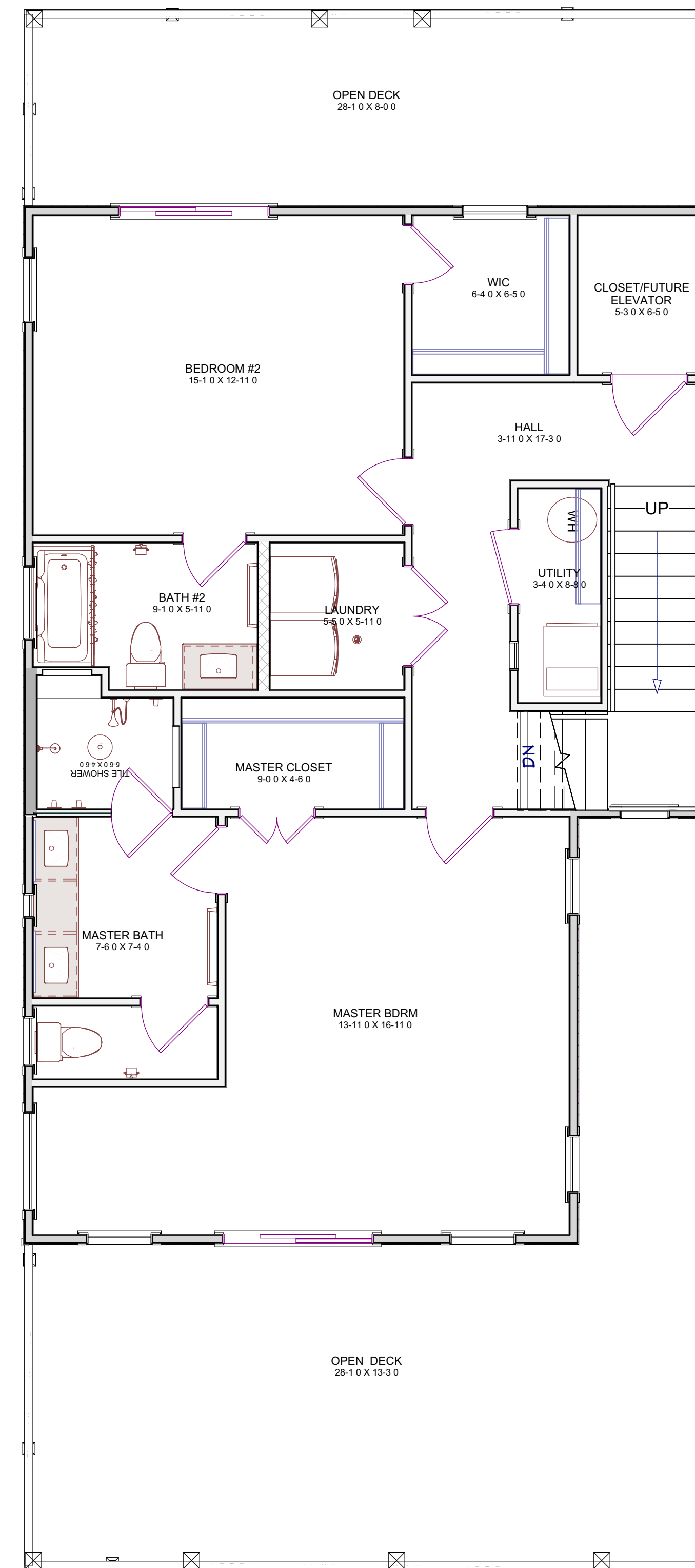
SECOND FLOOR
