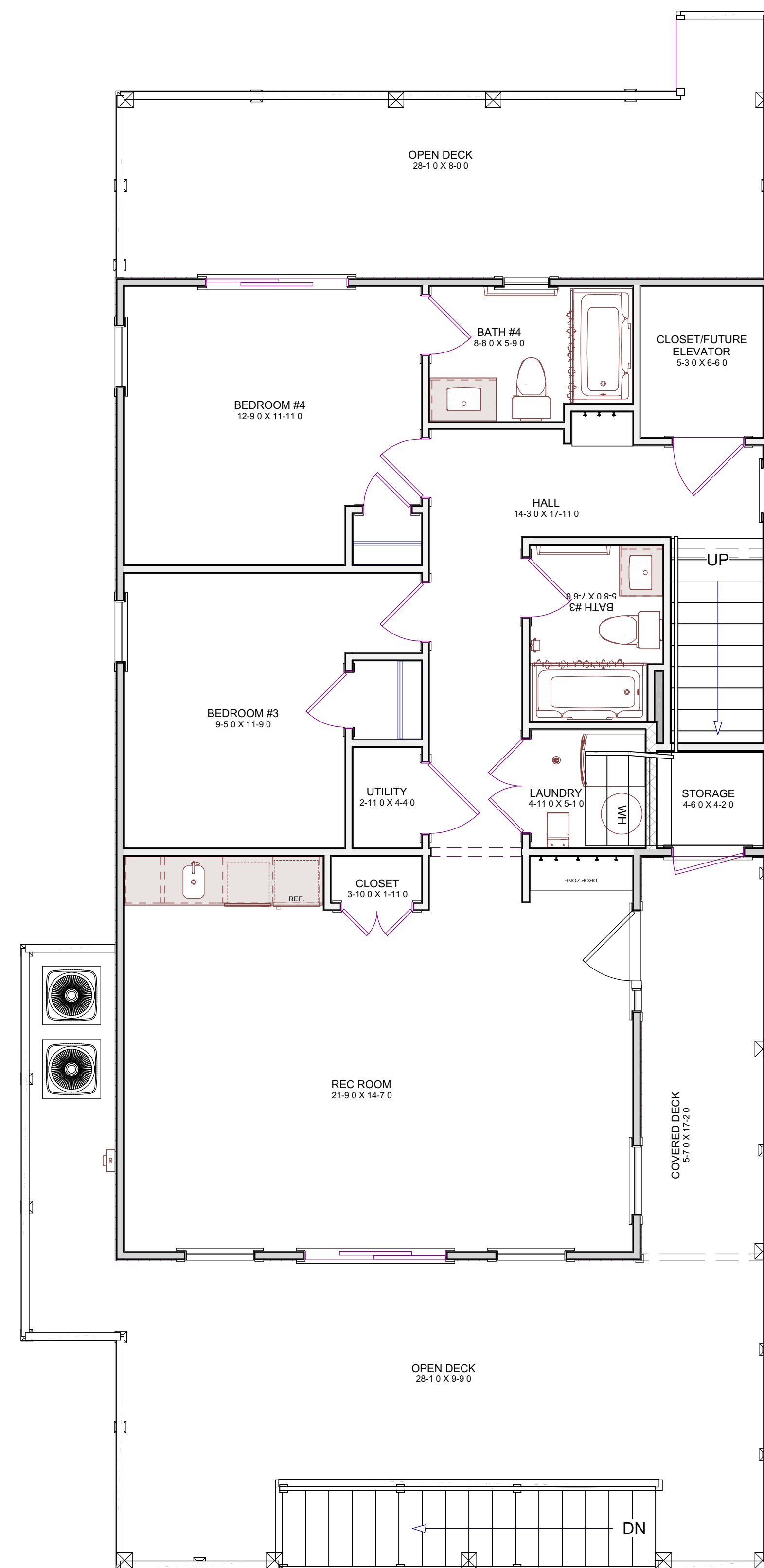
FIRST FLOOR
