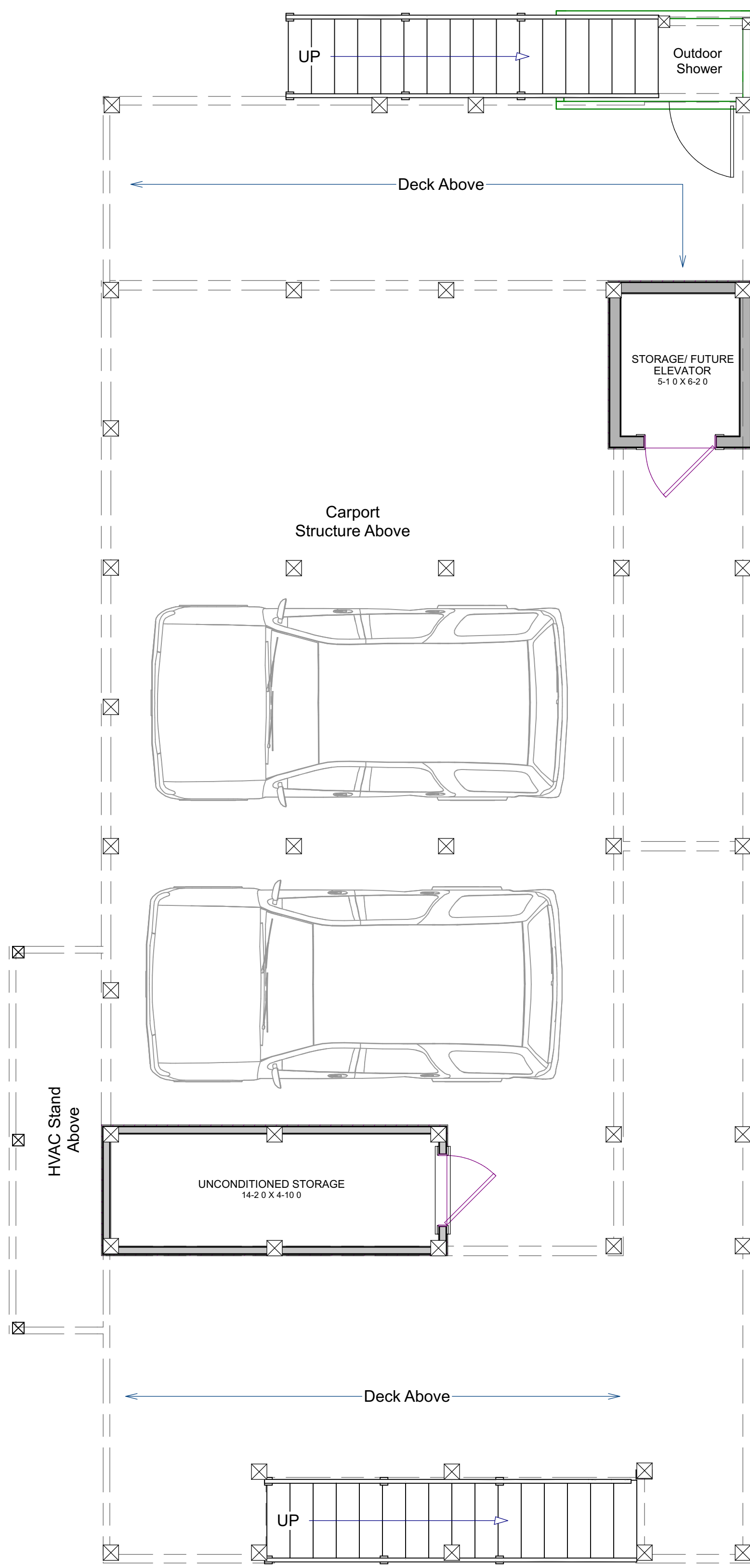
GROUND FLOOR
